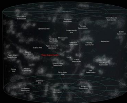
Local Superclusters
