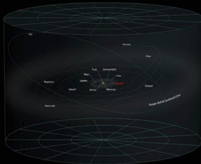
Solar System
