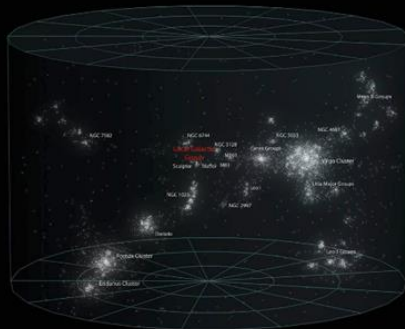
Virgo Supercluster
